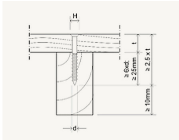
Image 5: The recommended point side penetration of screws into the sub-frame is at least 25mm, 6 x shank diameter or 1.5 x board thickness (whichever is the largest).
